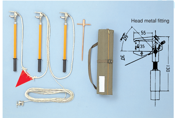
Model F (Universal type for cubicles) for 6.6~22kV c/w Carrying case
