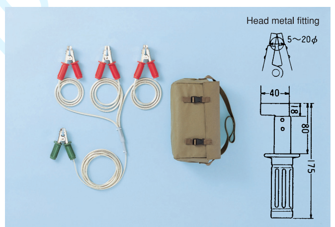
Model H (Universal type for cubicles) for 6.6kV c/w Carrying case
